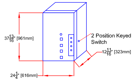
Soft Starter Control Panel
